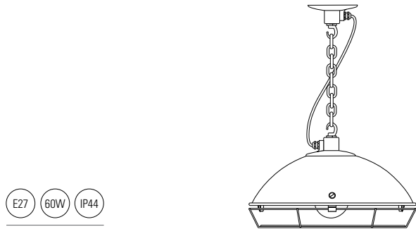
DP7242/GA/1ES/IP44 Cargo Cluster Light With Protective Guard, 1xE27, Galvanised, IP44
